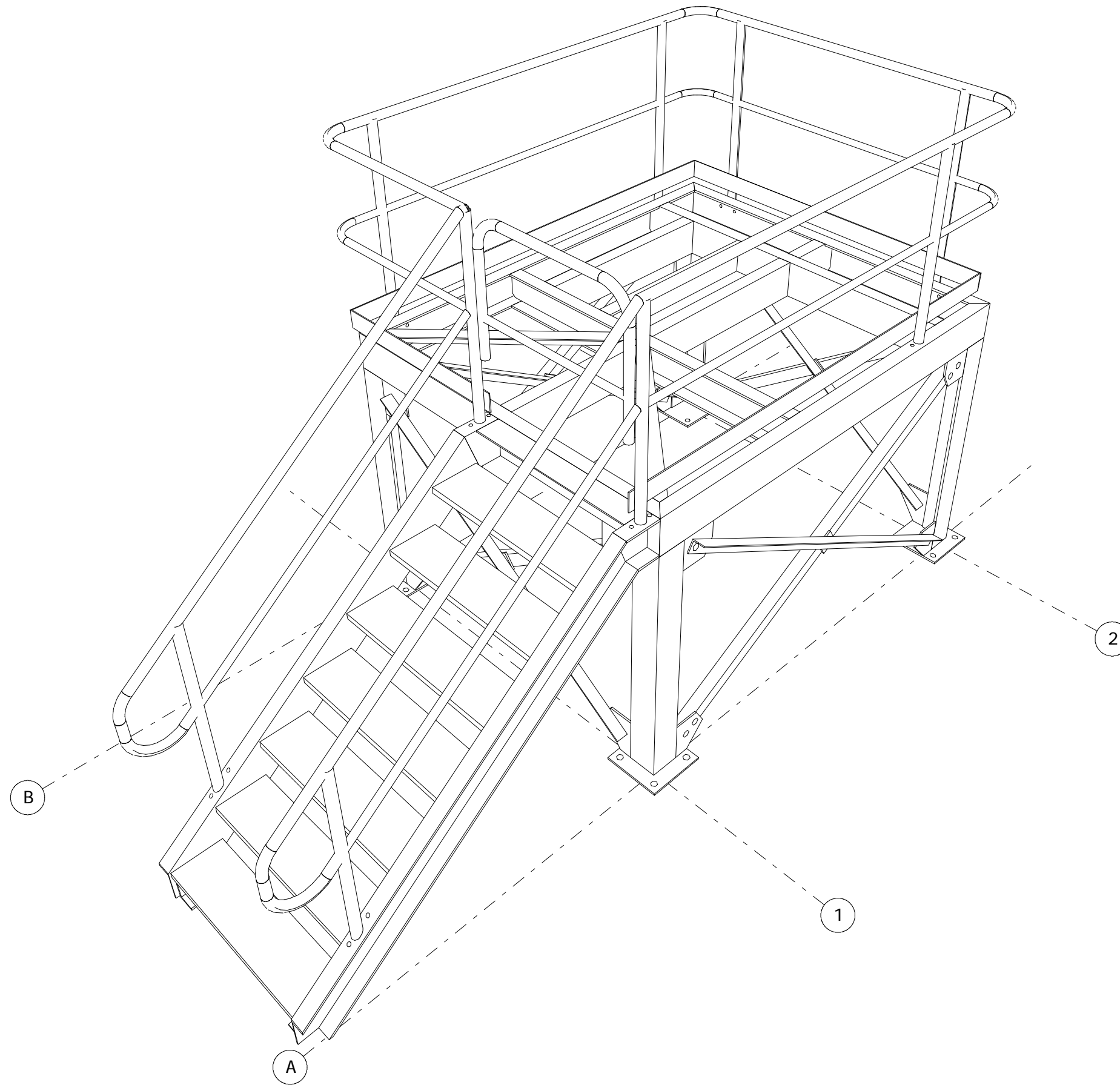
3-D VIEW
